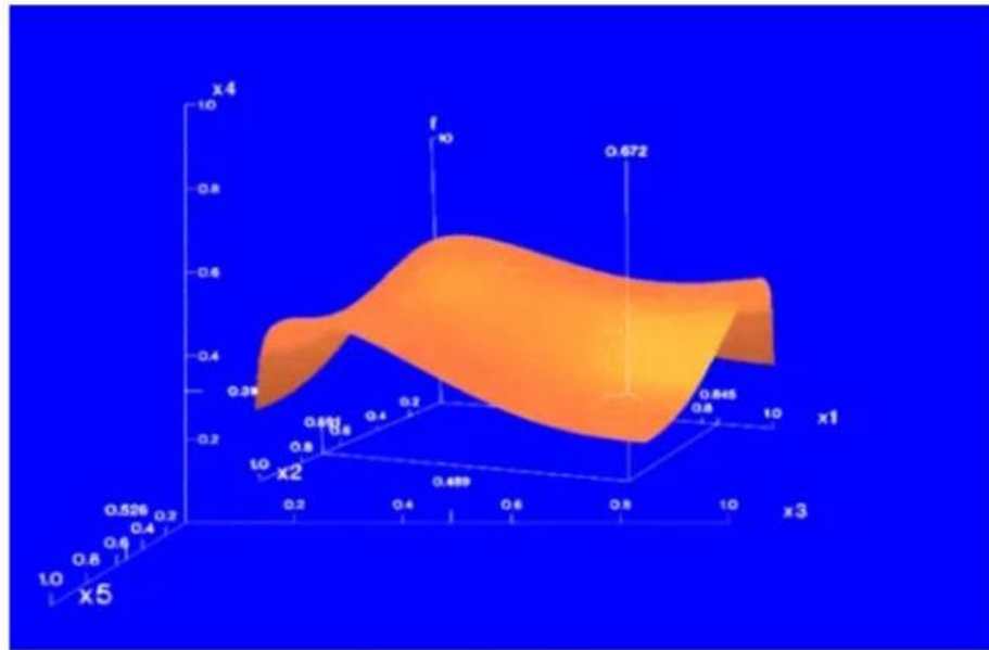
Hierarchical Visualization
